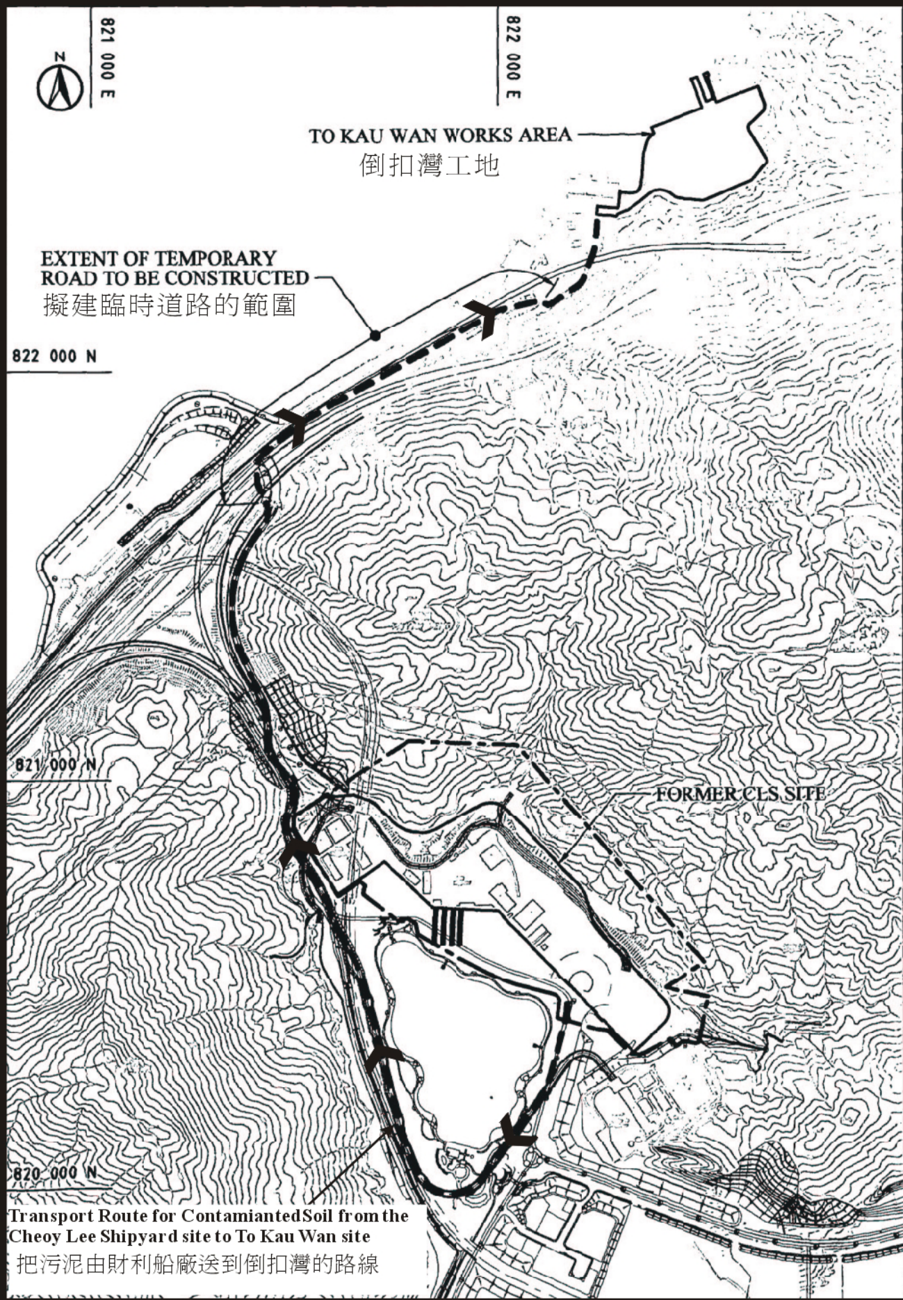
Fig. 5 Transport Route for Contaminated Soil from the Cheoy Lee Shipyard site to To Kau Wan site
